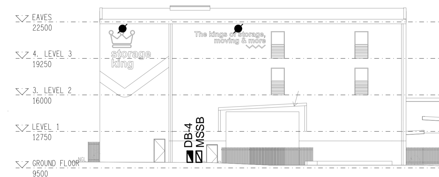
NORTH EXTERNAL BUILDING ELEVATION SCALE 1: 200
