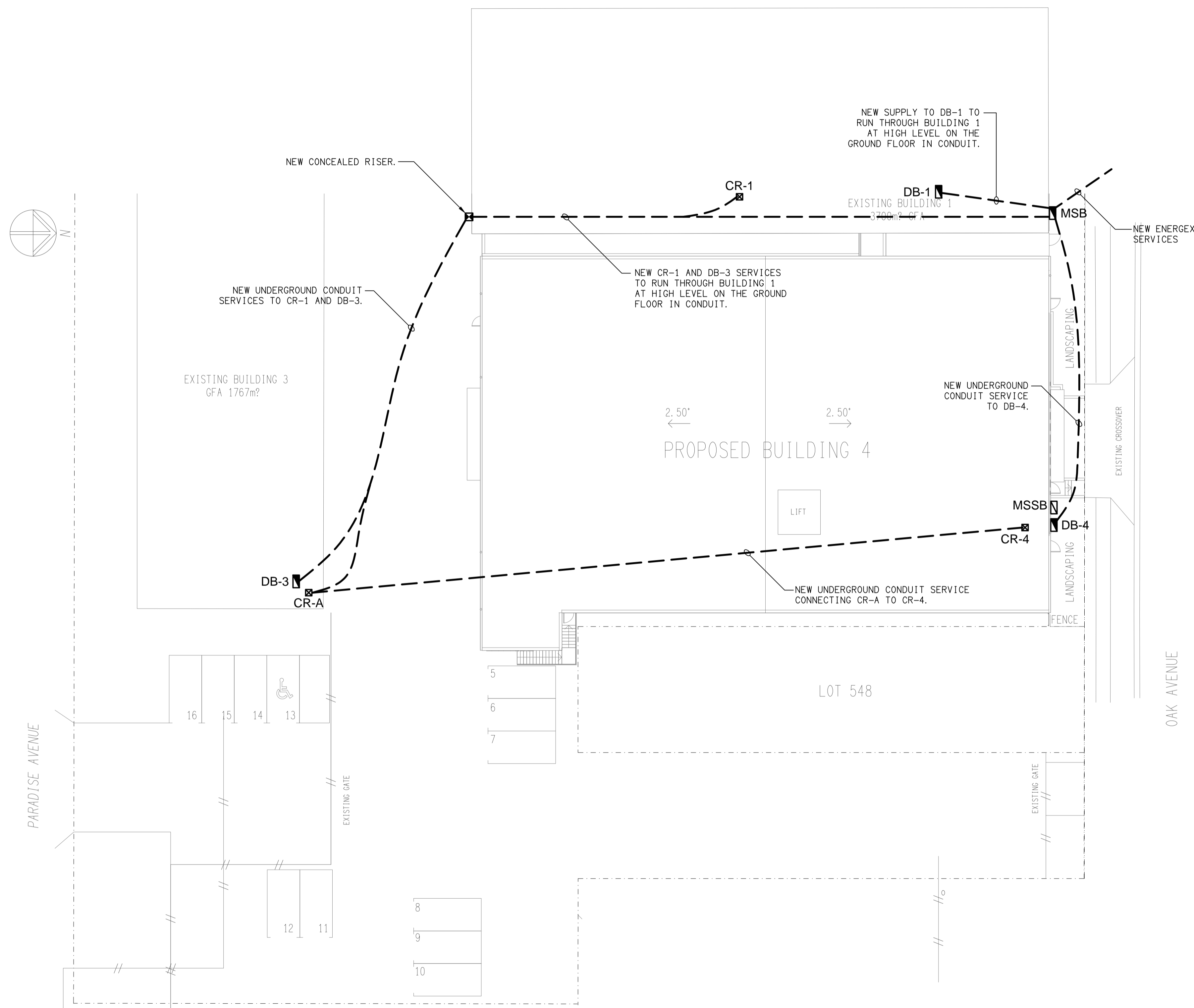
SITE PLAN PROPOSED BUILDING 4 SCALE 1: 200
