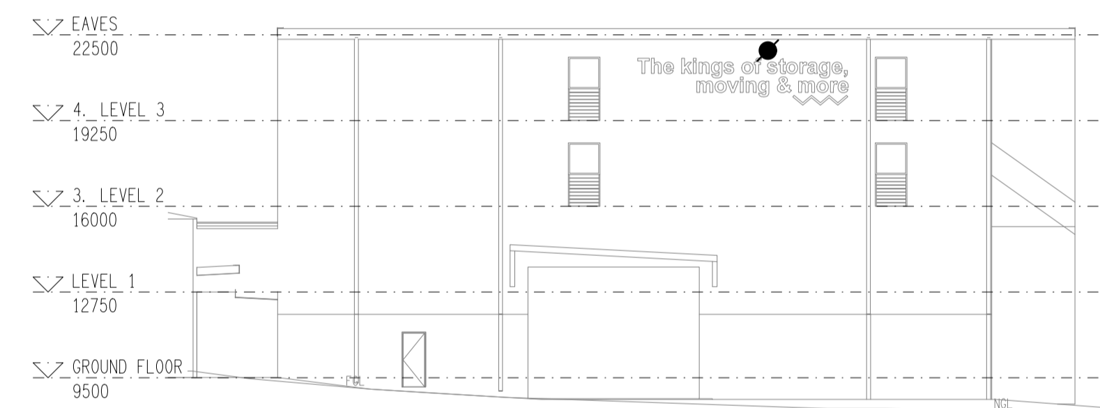
SOUTH EXTERNAL BUILDING ELEVATION SCALE 1: 200
