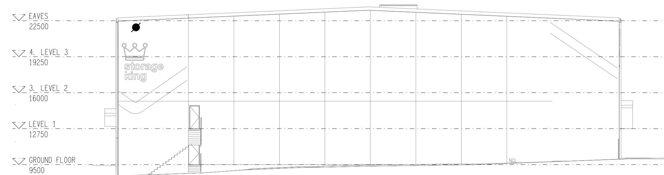
EAST EXTERNAL BUILDING ELEVATION SCALE 1: 200
